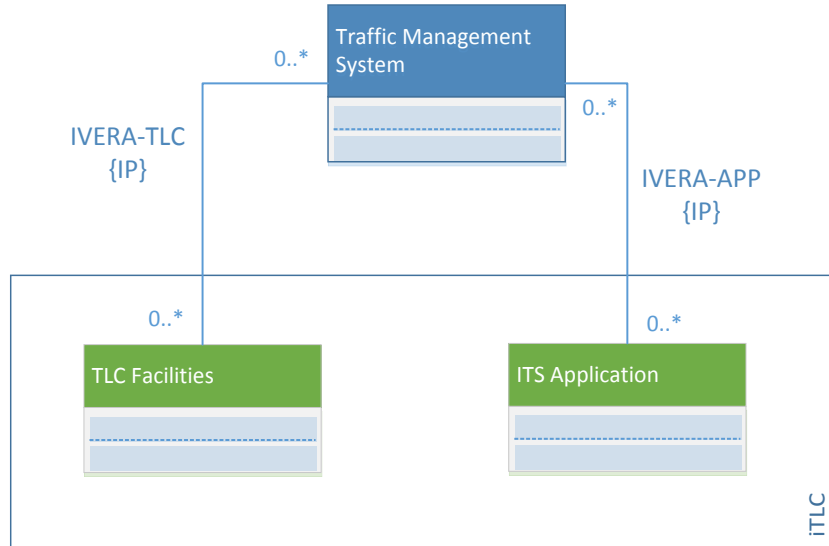
Figure 1 Functional model
